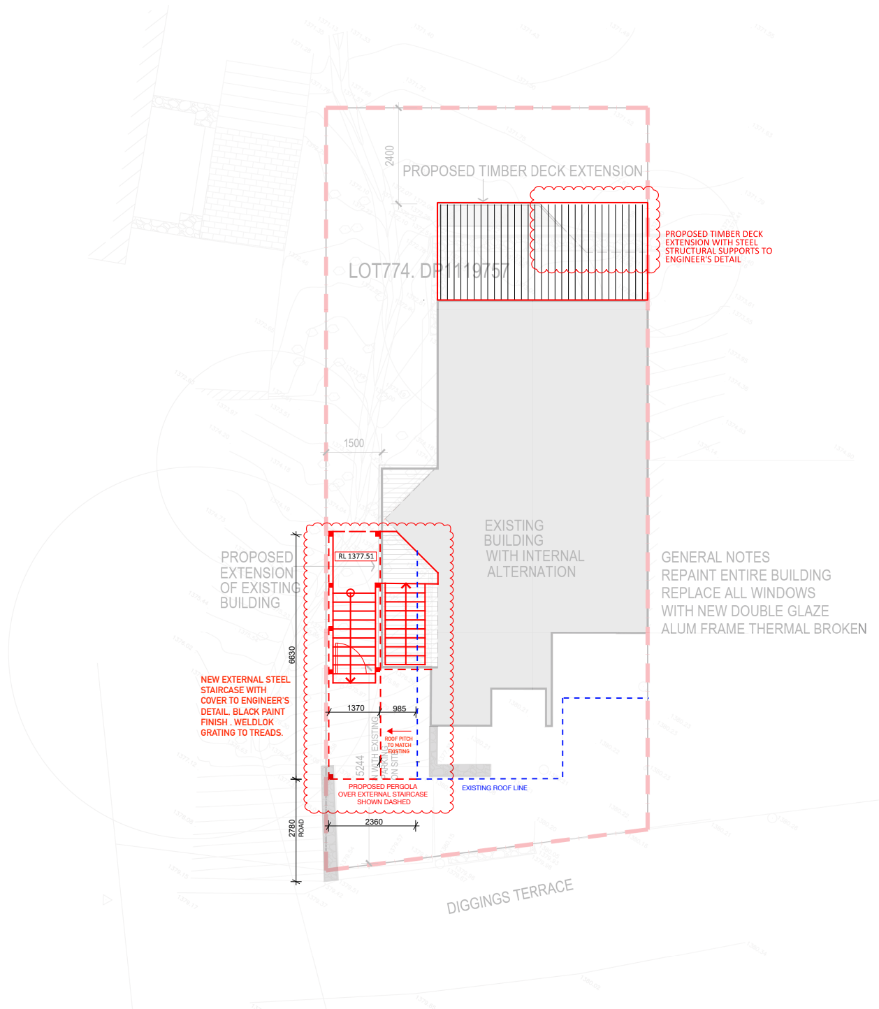
01 SITE PLAN SCALE 1:100 @ A3
